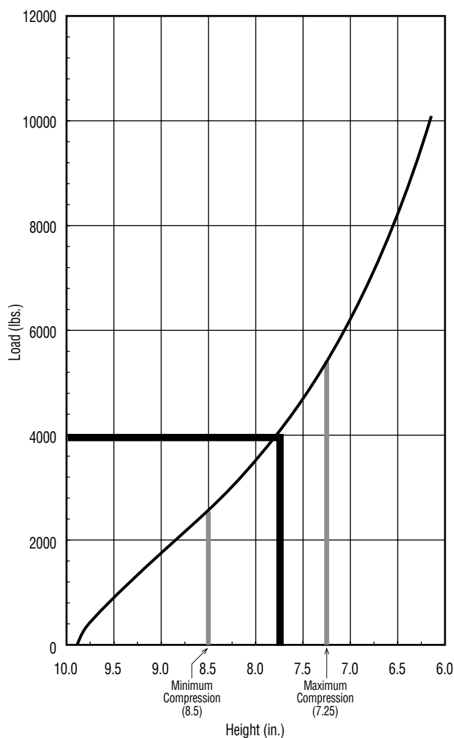
LOAD/DEFLECTION CURVE
